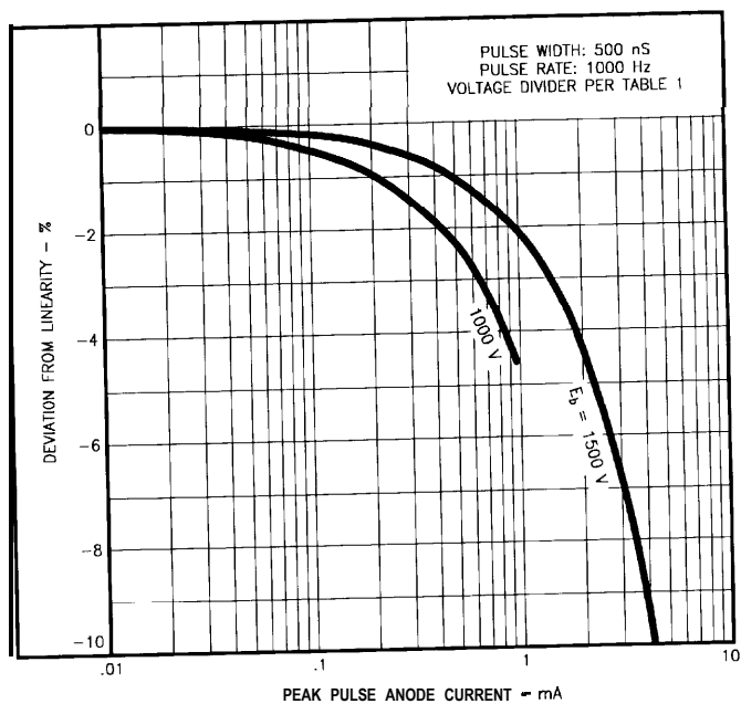
Figure 4 - Typical Anode Current Linearity Characteristics
