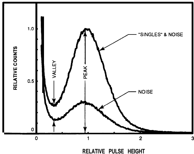
Figure 11 - Definition, Peak-to-Valley Ratio, Single Photoelectron Pulse Height Distribution
